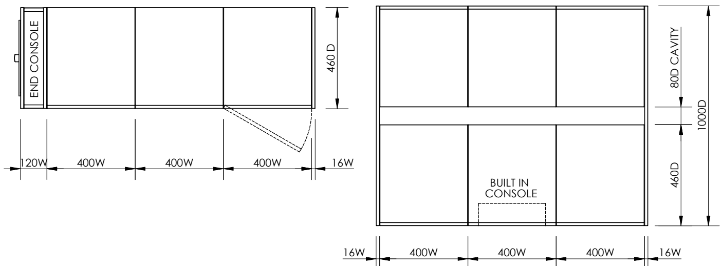
All dimensions shown in Millimetres (mm).
